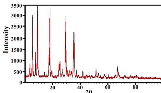
Fig. 6 X-ray powder diffraction pattern of [\text{Cu}(\text{ASA})_2] .
