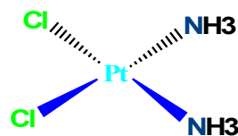
Fig. 1 Structure of Cisplatin
