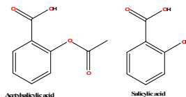
Fig. 2 Structure of acetylsalicylic acid and salicylic acid
