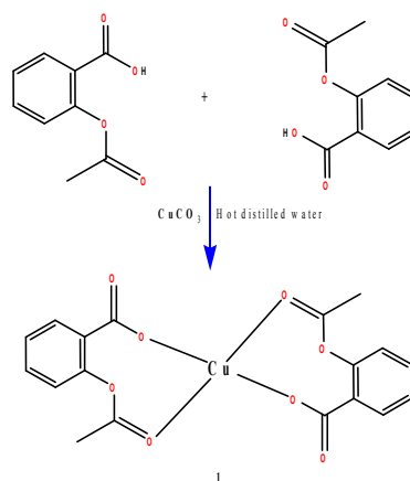
Fig. 3 Schematic synthesis of [Cu(ASA)_2] complex
