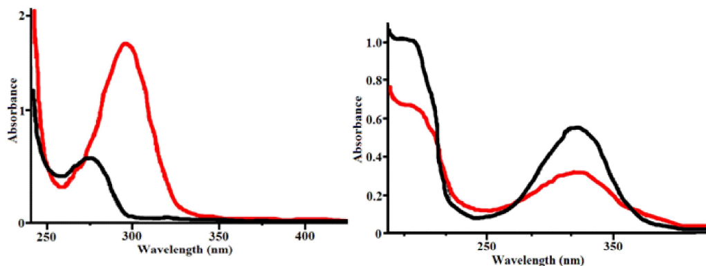
Fig. 5 Absorption spectra of aqueous solution of complexes 1 and 2 .
