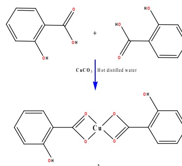
Fig. 4 schematic synthesis of [Cu(salH)_2] complex
